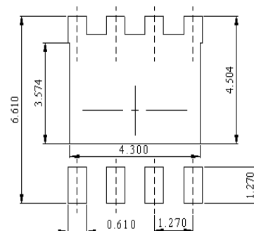
DIMENSIONS:MILLIMETERS
