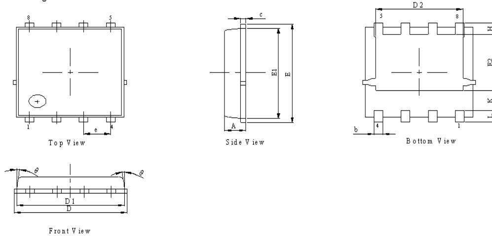
Package Outline
